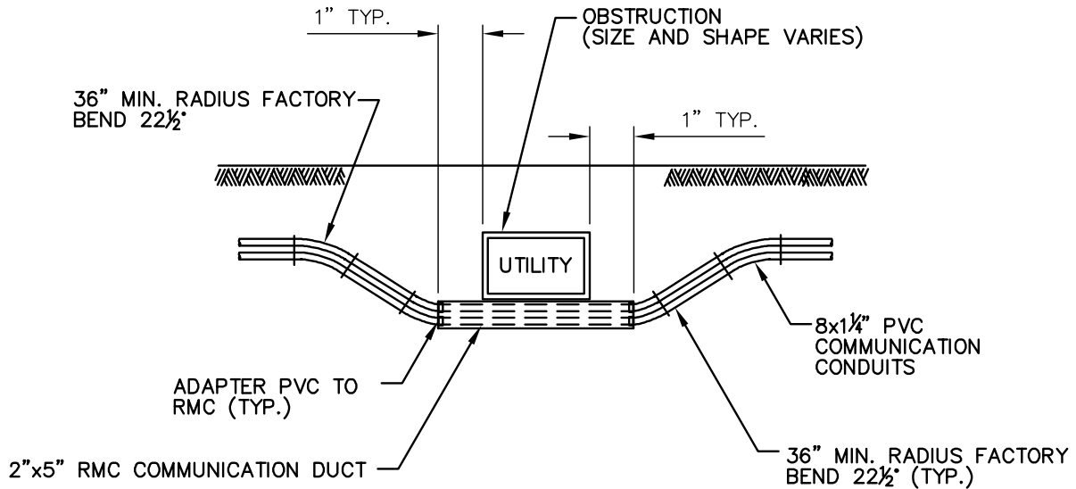
SECTION B-B
